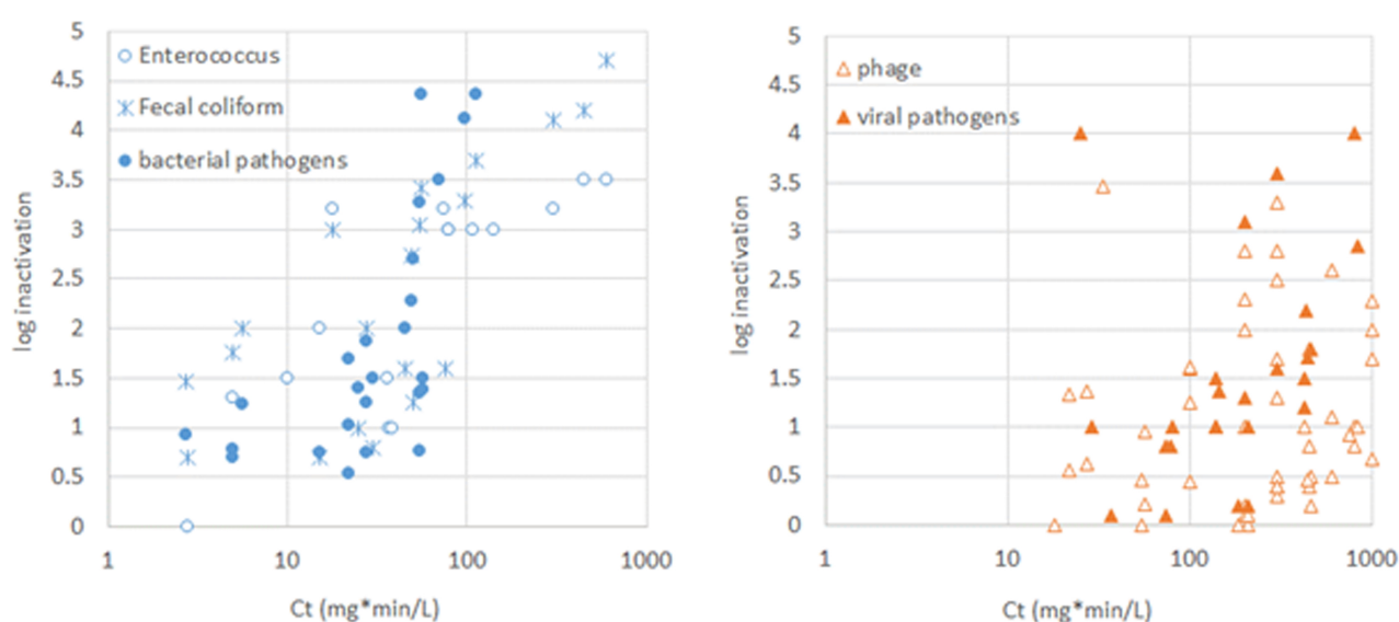
Figure 5. Comparison of the disinfection behavior of indicators ( Enterococcus and fecal coliform for bacteria; coliphages for virus) and corresponding pathogen groups during wastewater disinfection by chlorine.
