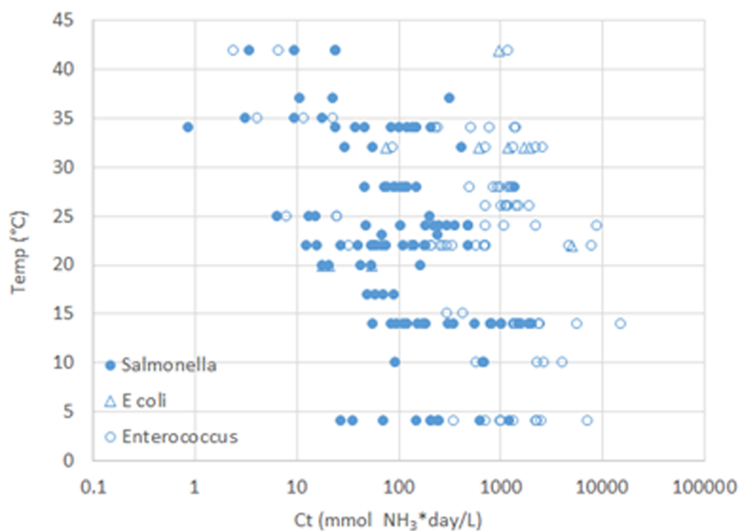
Figure 12. \text{NH}_3 exposure ( \text{NH}_3 concentration* T_{99} ) required to reach a 2 \log_{10} inactivation of bacteria as a function of the treatment temperature.
