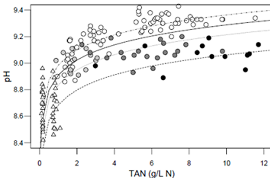
Figure 7. pH of fecal sludge after addition of different doses of urea, expressed as total ammonia nitrogen (TAN) and as a function of total solids content. White dots: 0.2% solids; light grey dots: 0.4% solids; dark grey dots: 0.7-1.2% solids; black dots: 3-5% solids. White triangles are treatments with decreasing pH. The lines represent model fits to the data as explained in Fidjeland, 2015 (Figure source: Fidjeland, 2015).
