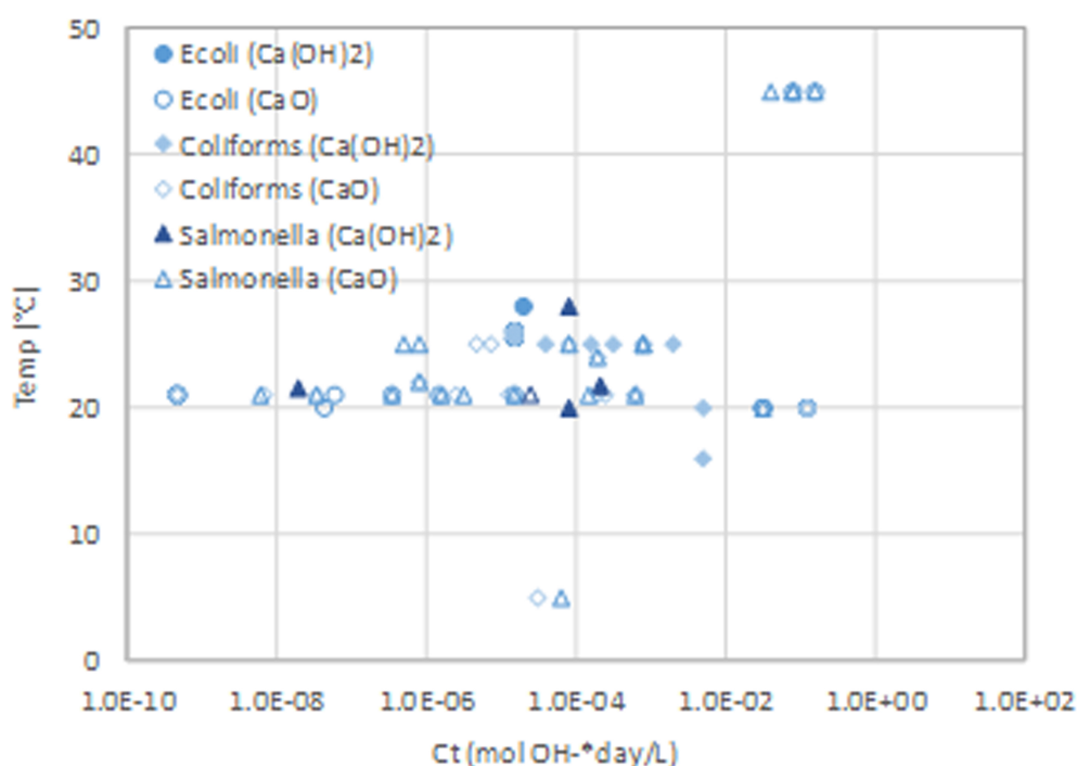
Figure 17. Lime exposure ( \text{OH}^- concentration added* T_{99} ) needed to achieve a 2 \log_{10} inactivation of E. coli , coliforms (including faecal coliforms) and Salmonella spp., as a function of temperature and type of lime added.
