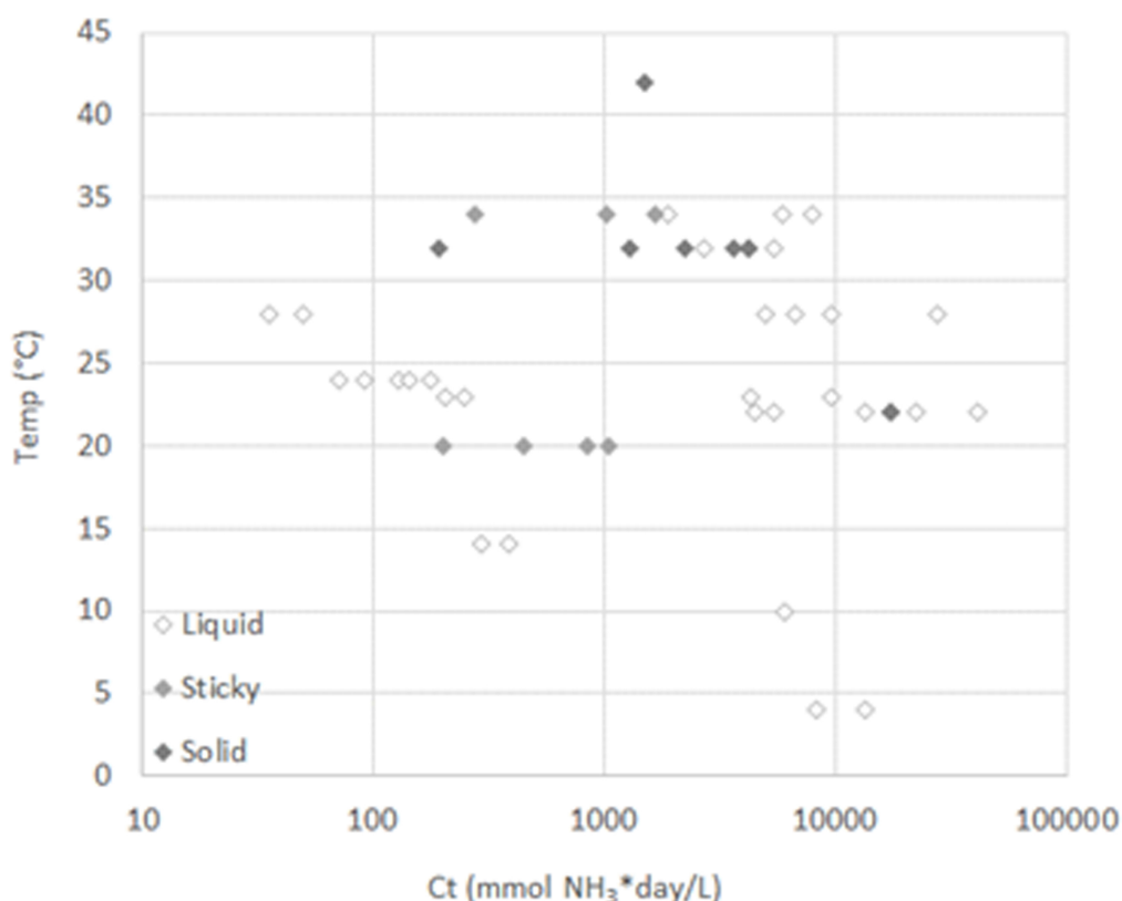
Figure 13. \text{NH}_3 exposure ( \text{NH}_3 concentration* T_{99} ) required to reach a 2 \log_{10} inactivation of Ascaris , as a function of solids content and temperature of the matrix. Note that the effect of solids on pH, and hence \text{NH}_3 content, is not visible from this graph, as these effects are accounted for by using Ct, rather than added ammonia, on the x-axis.
