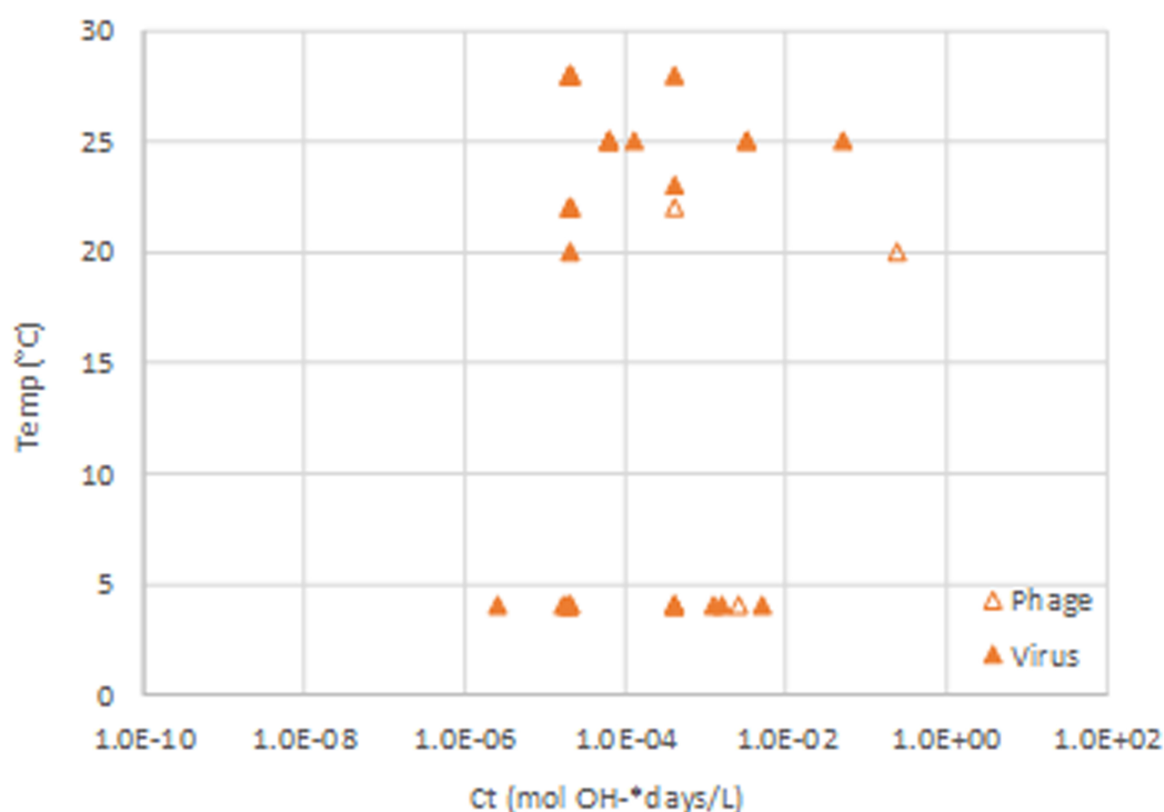
Figure 18. Lime exposure ( \text{OH}^- concentration added* \text{T}_{99} ) needed to achieve a 2 \log_{10} inactivation of mammalian viruses and phages as a function of temperature.
