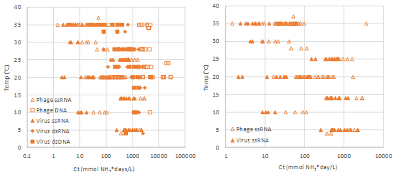
Figure 11. \text{NH}_3 exposure ( \text{NH}_3 concentration* T_{99} ) required to reach a 2 \log_{10} inactivation of mammalian viruses and bacterial phages as a function of the treatment temperature. Left panel: all genome types. Right panel: ssRNA viruses and phages only.
