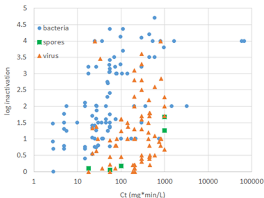
Figure 1. Overview over reported data on chlorine disinfection of bacteria, spores and viruses in waste-water and sludge matrices. For those studies that did not report measured exposures, Ct was estimated from the reported applied or measured chlorine concentrations and treatment times. The references used to create this plot are indicated in the reference section.
