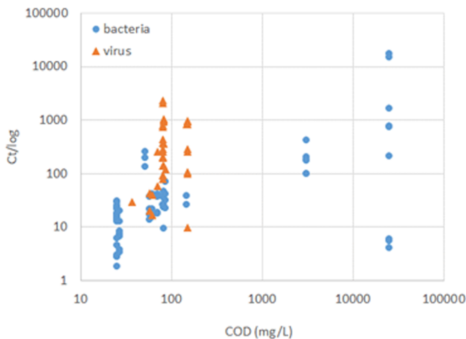
Figure 3. Required Ct (mg*min/L) to achieve a 1 log 10 pathogen reduction, as a function of the chemical oxygen demand of the matrix. If COD was not reported, it was estimated based on total organic carbon (TOC) or bioavailable organic carbon (BOD), using the ratios COD/TOC = 3 and COD / BOD = 2.1 (Fuller, 2016, accessed 2016).
