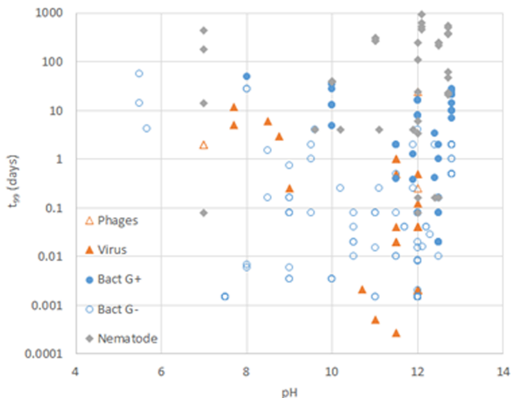
Figure 14. Time needed to achieve a 2 log 10 inactivation (T 99 ) of different organisms groups (phages, mammalian virus, gram positive bacteria (Bact G+), gram negative bacteria (Bact G-) and nematodes), as a function of pH. The references used to create this plot are indicated in the reference section.
