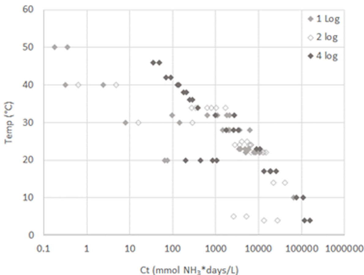
figure 10. \text{NH}_3 exposure ( \text{NH}_3 concentration* T_{99} ) required to reach a 1, 2, or 4 \log_{10} inactivation of Ascaris spp. as a function of the treatment temperature.
