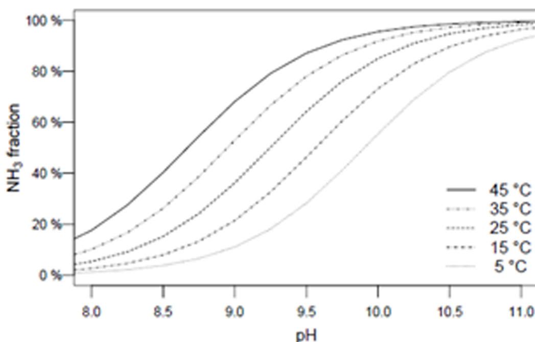
Figure 6. NH 3 (aq) fraction of total aqueous ammonia (NH 3 +NH 4 + ), plotted as a function of pH and temperature, based on equilibrium calculation according to Emmerson.
